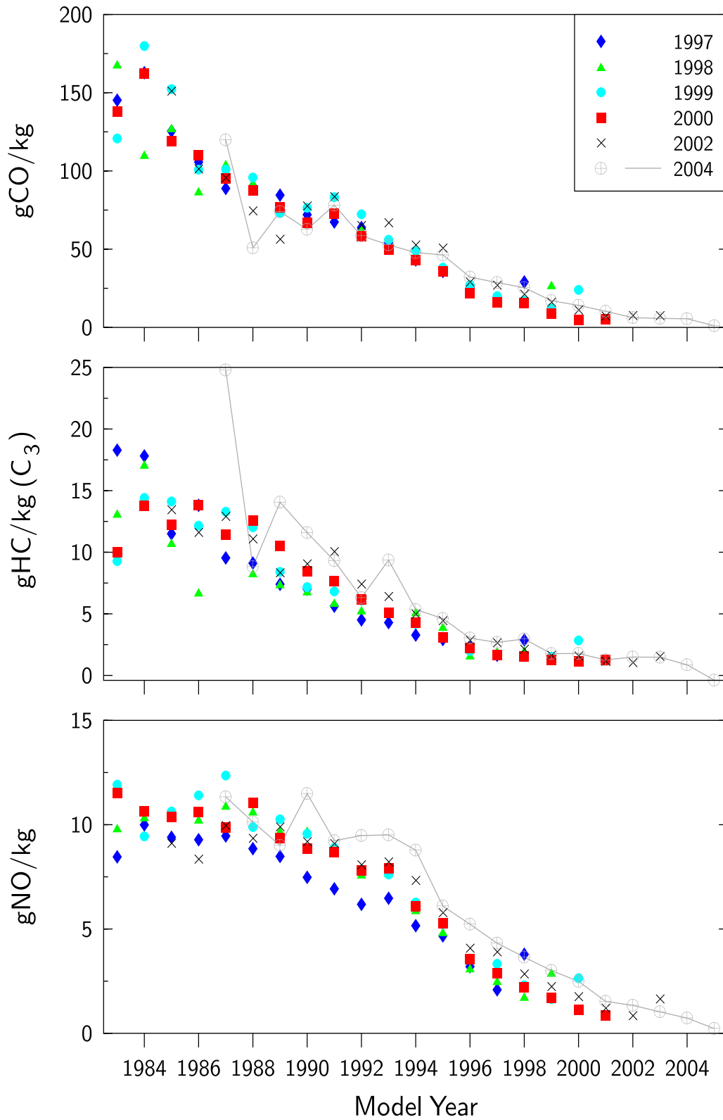
Figure 4. Mean vehicle emissions illustrated as a function of model year. HC data have been offset adjusted as described in the text.
