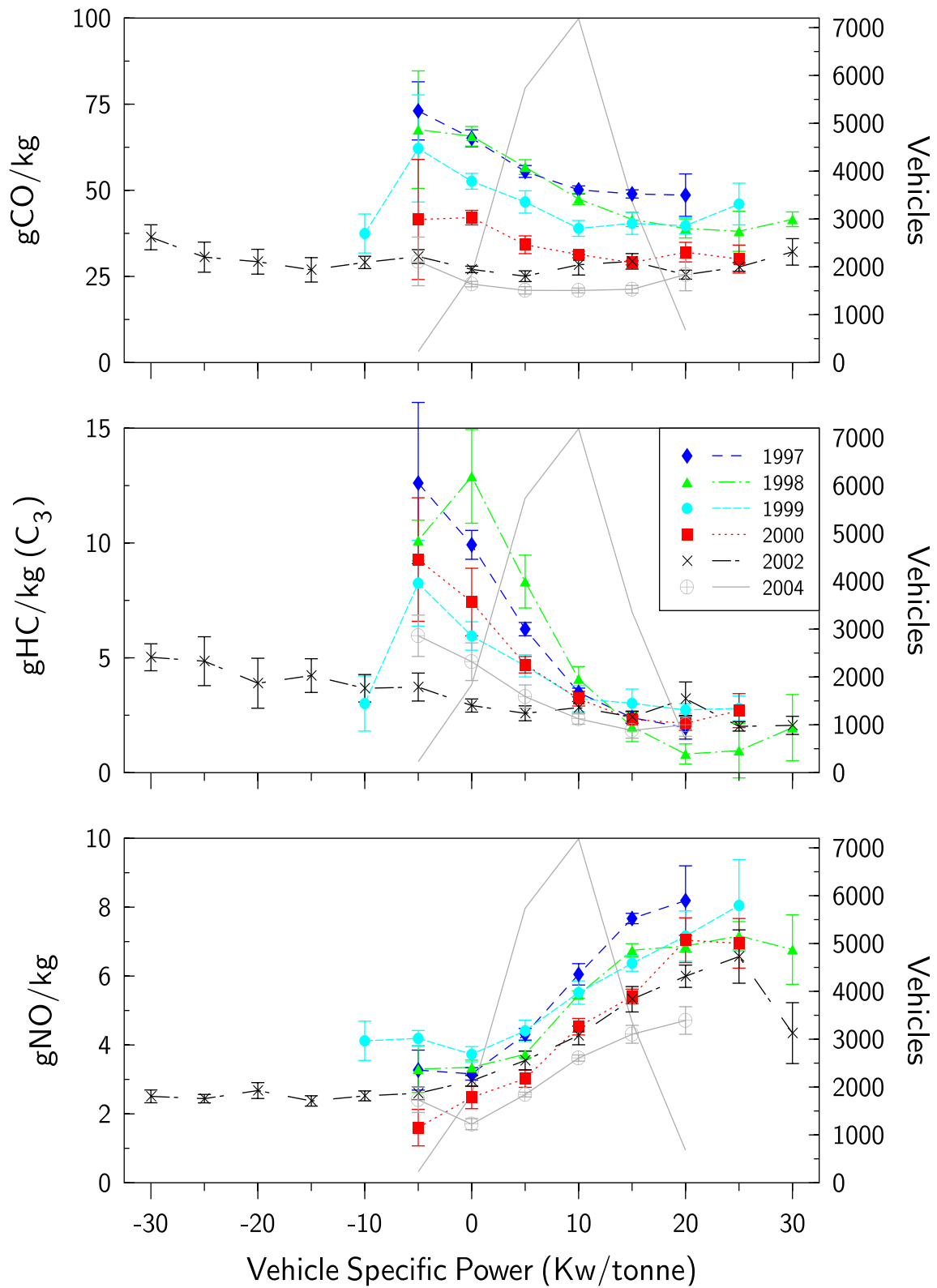
Figure 8. Vehicle emissions as a function of vehicle specific power for all of the Chicago E-23 data sets. Error bars are standard errors of the mean calculated from daily samples. The solid line without markers is the vehicle count profile for the 2004 data set.
