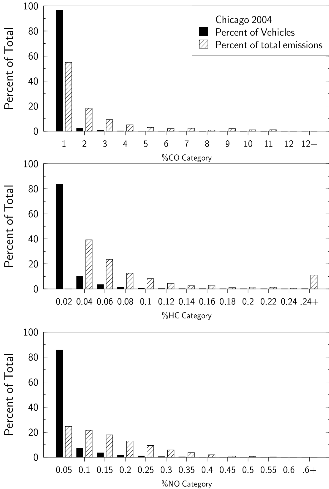
Figure 3. Emissions distribution showing the percentage of the fleet in a given emissions category (black bars) and the percentage of the total emissions contributed by the given category (shaded bars).
