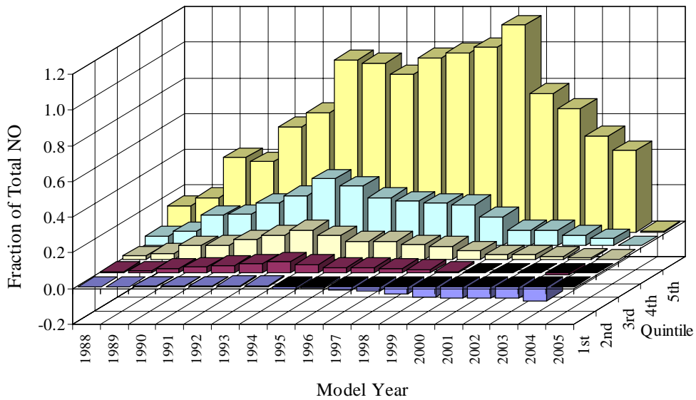
Figure 7. 2004 NO emissions by model year and quintile (top), fleet distribution (middle) and their product showing the total fractional NO emissions by model year and quintile (bottom).
