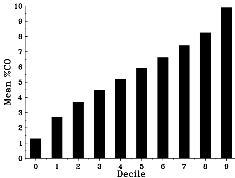
Figure 2. Mean %CO emissions by decile for all valid CO and HC measurements (1212 sleds) collected at the W. Yellowstone entrance to Yellowstone National Park.
