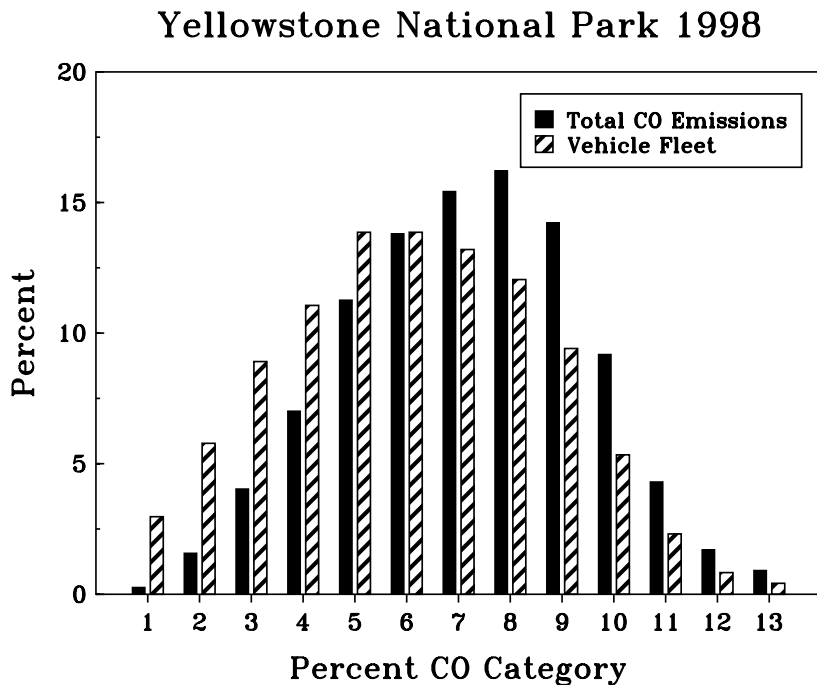
Figure 1. Percent of snowmobile fleet and the total CO emissions for all valid CO and HC measurements (1212 sleds). The upper boundary of each bin defined as \leq %CO.
