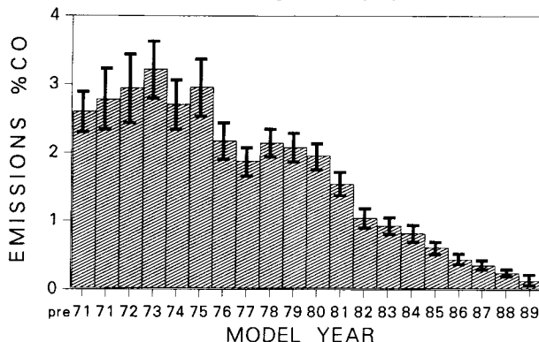
Figure 2. Emission factors by model year for all of the video data from both sites, regardless of fuel oxygenation; 4909 vehicles measured. Error bars are \pm 1 SEM.
